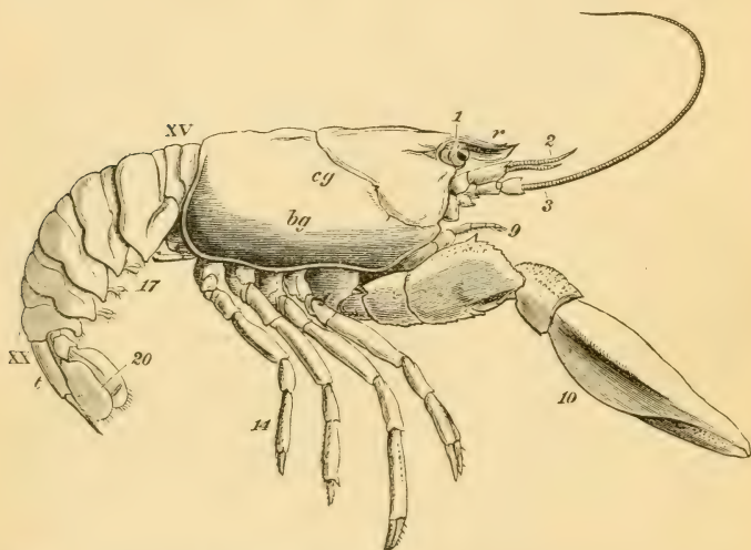
FIG. 1.— Astacus fluvialilis .—Side view of a male specimen (nat. size):— bg , branchiostegite; cg , cervical groove; r , rostrum; t , telson.—1, eye-stalk; 2, antennule; 3, antenna; 9, external maxillipede; 10, forceps; 14, last ambulatory leg; 17, third abdominal appendage; 20, lateral lobe of the tail-fin, or sixth abdominal appendage; XV, the first; and XX, the last abdominal somite. In this and in succeeding figures the numbers of the somites are given in Roman, those of the appendages in ordinary numerals.
